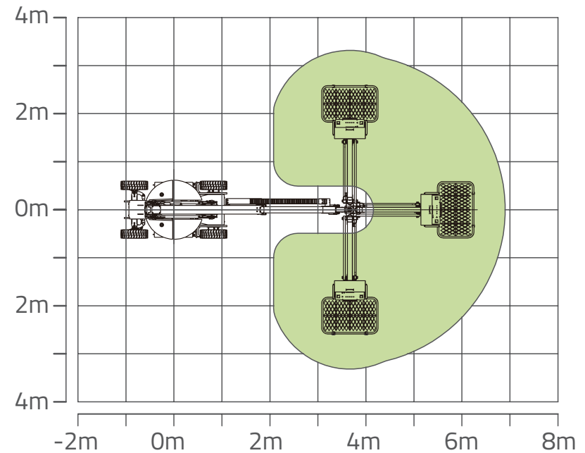
Range of Jib Swing Motion ZA10RJE
